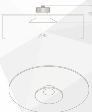
CupBouncer
